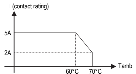
Contact Current rating vs Operating Ambient Temperature:
